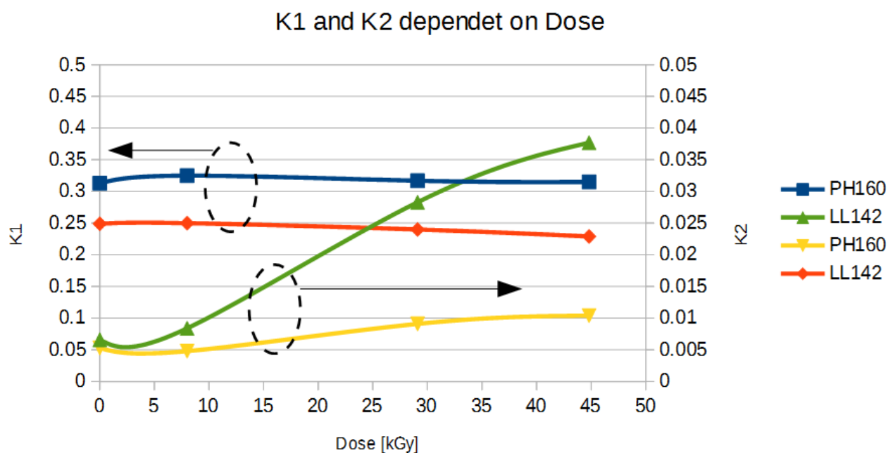
Figure 5: Coaxial-Cable parameters dependent on irradiation dose
